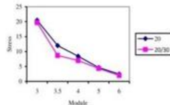
Graph 7 comparisons of equivalent stresses between symmetric (20°) and asymmetric (20/30°) spur gears with different modules
