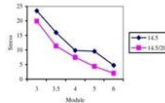
Graph 6 comparisons of equivalent stresses between symmetric (14.5°) and asymmetric (14.5/20°) spur gears with different modules
