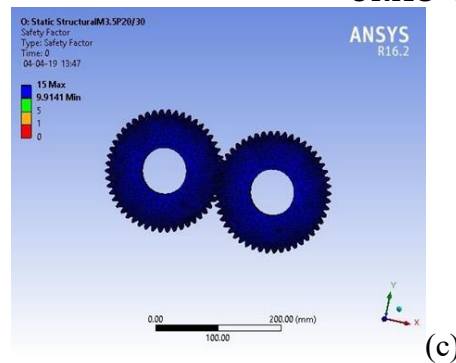
Fig.5 (a) equivalent stress ; (b) Total deformation; (c) safety factor of spur gear with module 3.5 and pressure angle 20
