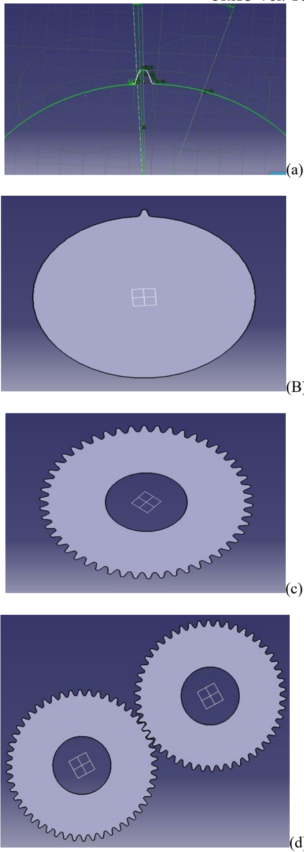
Fig. 1 (a)showing tooth profile in catia; (b)tooth profile after pad option; (c)tooth profile with 50 teeth; (d)assembly of spur gears
