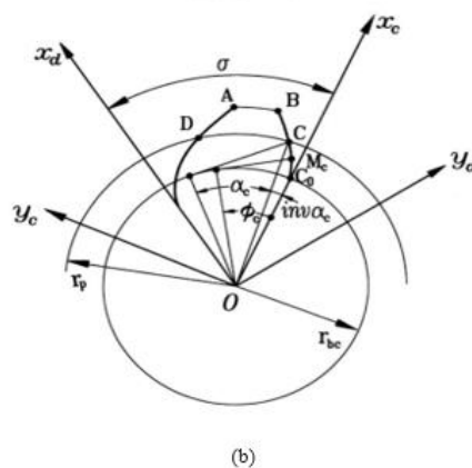
Fig.3 (a) Representation of drive profile; (b) Representation of coast profile.
