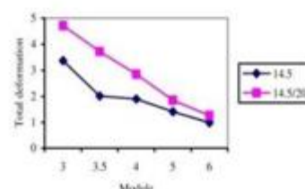
Graph 8 comparisons of total deformation between symmetric (14.5°) and asymmetric (14.5/20°) spur gears with different modules
