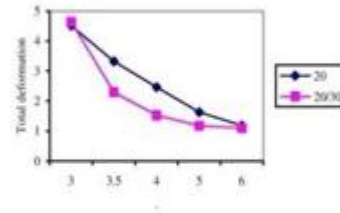
Graph 4 comparison of total deformation between symmetric (20°) and asymmetric (20/30°) spur gears with different modules
