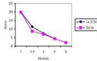
Graph 3 Comparison of equivalent stresses between two different asymmetric spur gears (14.5/20°) (20/30°) with different modules
