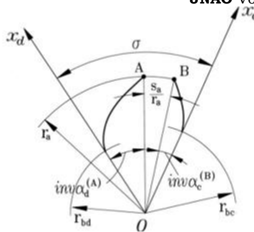
Fig.4 Determination of addendum tooth tip thickness
