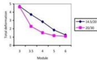
Graph 5 comparisons of total deformation between two different asymmetric spur gears (14.5/20°) (20/30°) with different modules
